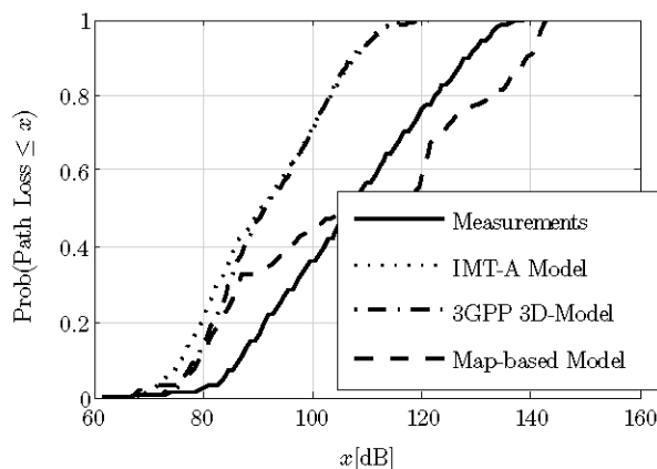
Fig. 4. CDF of the path loss values in the area under study.
