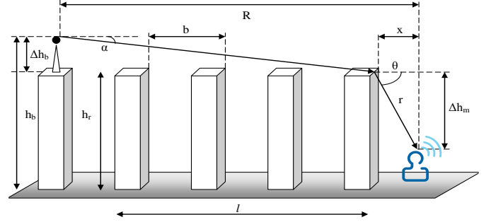
Fig. 1. Geometry of the large scale model.
