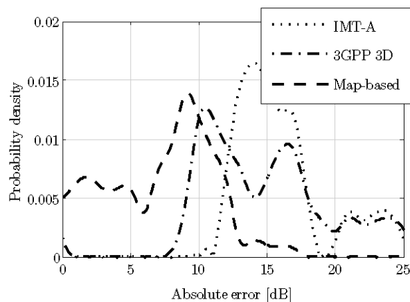
Fig. 5. Probability distribution of the absolute error in the path loss estimation.
