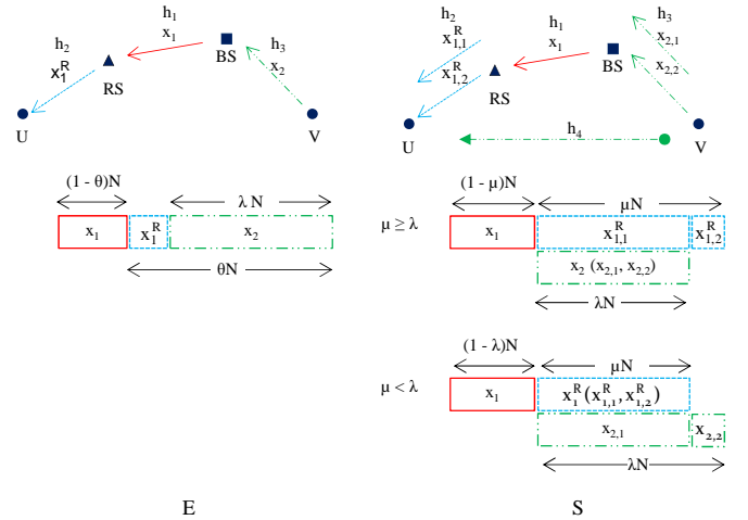
Fig. 1. Reference E and S CDR Schemes. In each scheme, the time interval of the transmission represented by an arrow above is represented by a rectangular below with the same color and the transmissions represented by the rectangles in the same column are conducted simultaneously.
