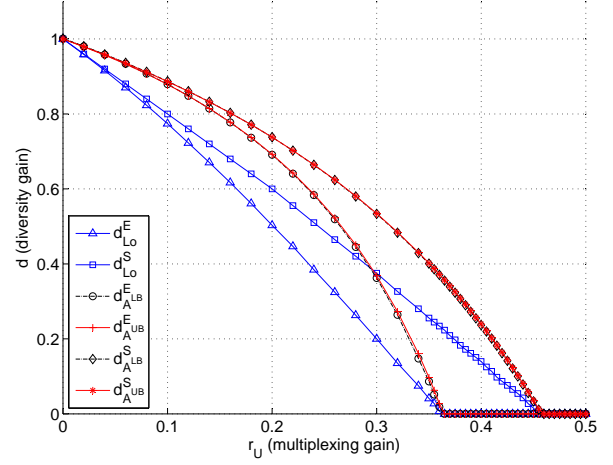
Fig. 4. The optimal DMT functions of E and S in CSI-L, d_{Lo}(r) , and the lower and upper bounds of the DMT functions of E and S in CSI-A with r_V = \frac{3}{4}r_U and \beta = 2.3 .
