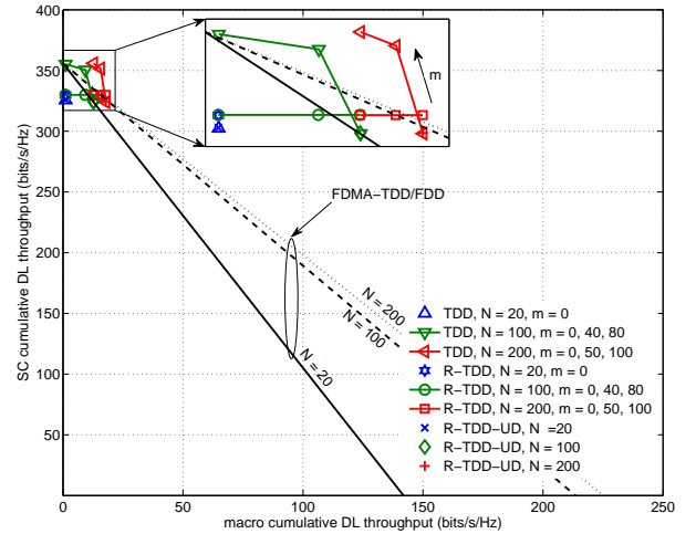
Fig. 5. Achievable DL rates of outdoor scenario. The connected points denote the achievable spectral efficiency of a scheme with increasing m from right to left.
