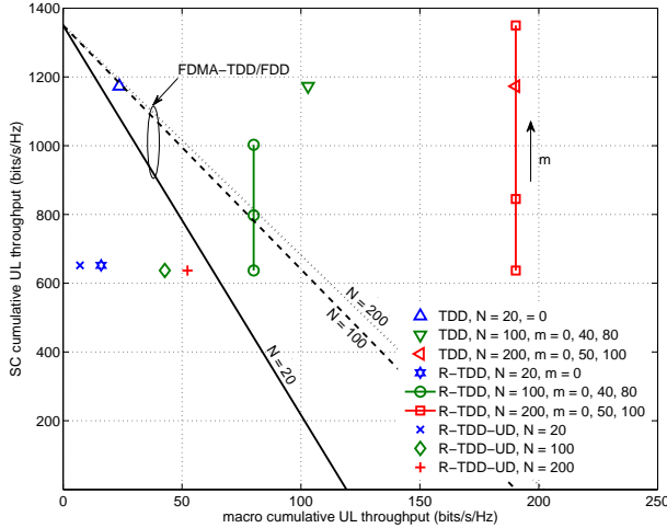
Fig. 6. Achievable UL rates of indoor scenario. The connected points denote the achievable spectral efficiency of a scheme with increasing m from bottom to top.
