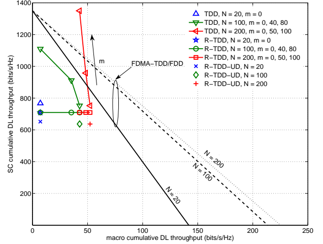
Fig. 4. Achievable DL rates of indoor scenario. The connected points denote the achievable spectral efficiency of a scheme with increasing m from right to left.
