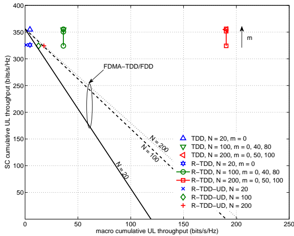
Fig. 7. Achievable UL rates of outdoor scenario. The connected points denote the achievable spectral efficiency of a scheme with increasing m from bottom to top.
